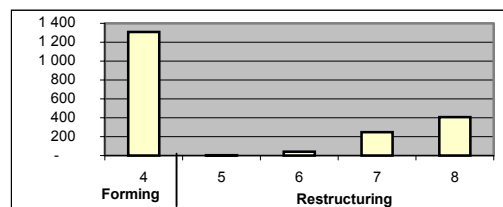
Figure 7. Size of messages sent (measured by number of sets) during a negotiation with 4 agents and classes varying from 4 to 8
