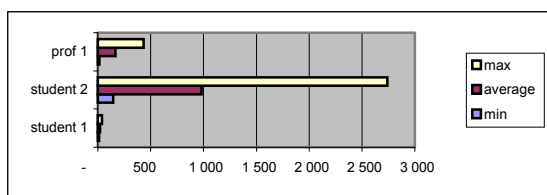
Figure 6. Total size of messages sent (measured by number of sets) during a negotiation with 4 agents and 4 tasks
