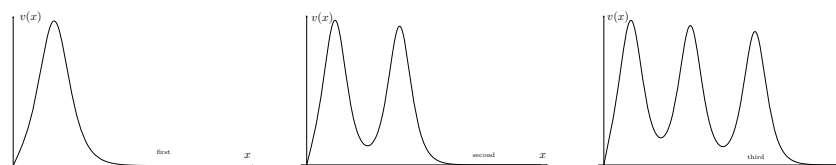
FIGURE 7. Functions corresponding to the first three turning points to the right in the bifurcation diagram, corresponding now to \varepsilon = 0.01 .
