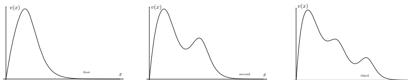
FIGURE 6. Functions corresponding to the first three turning points to the right in the previous bifurcation diagram, with \varepsilon = 0.2 , after the transformation:
