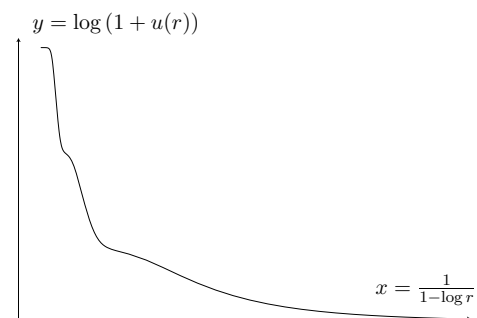
FIGURE 8. A 3-bubble solution u of (1.1) corresponding to the three bumps solution v of Figure 7, with \varepsilon = 0.01 . Appropriate scales have been chosen.
